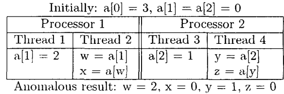
Figure 8: Interference by other threads on same processor
